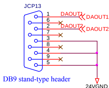
Analog voltage output interface
