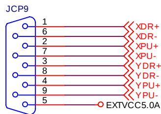
DB9 stand-type header
