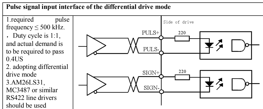
Pulse signal input interface of the differential drive mode
