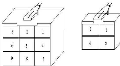
Encoder 9 pin
