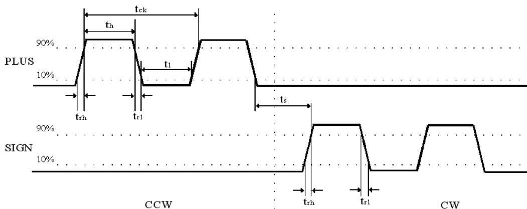
CW + CCW Pulse Input Interface Timing Diagram (Pulse Frequency ≤ 500kHz)
