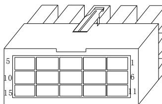
encoder Terminal
