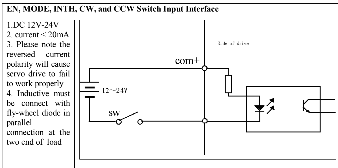
Switch Input Interface
