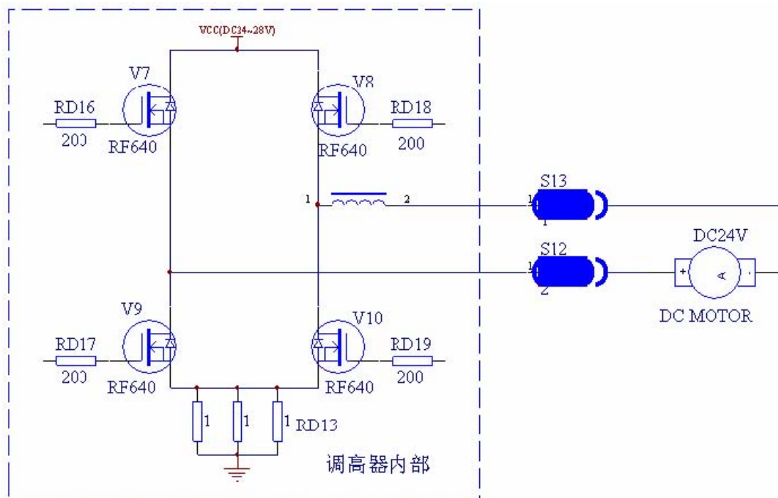
Figure 19: MOTOR drive
