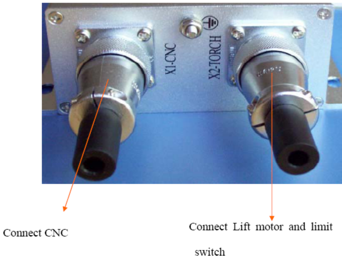
Figure 9: Back of CHC-200D
