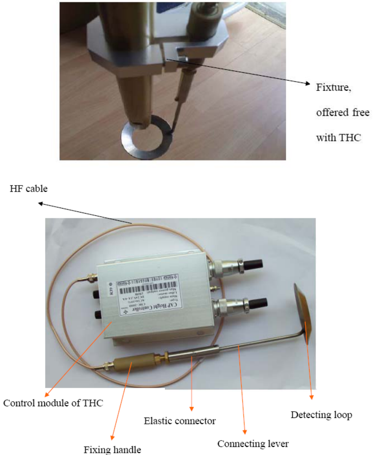
Figure 7 : CHC-200D Assembly
