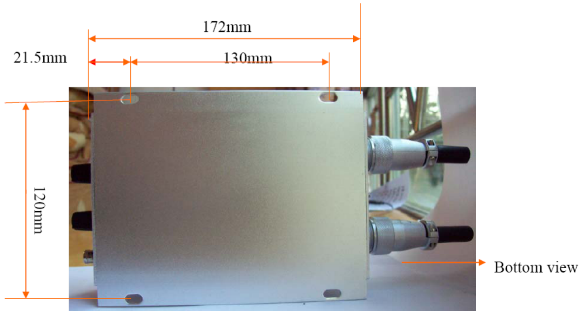
Figure 4 : Bottom view and installation size
