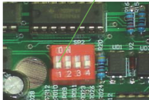
Figure 20: PWM frequency switch
