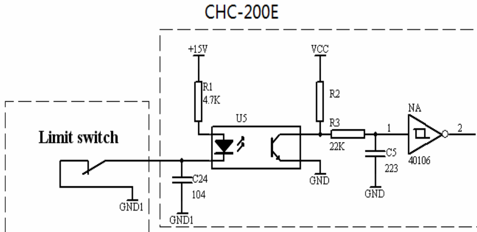
Figure 3-6 Limit input
