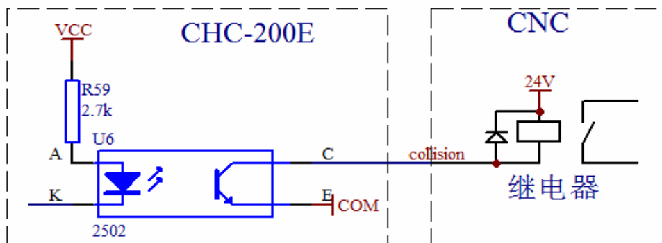
Output circuit
